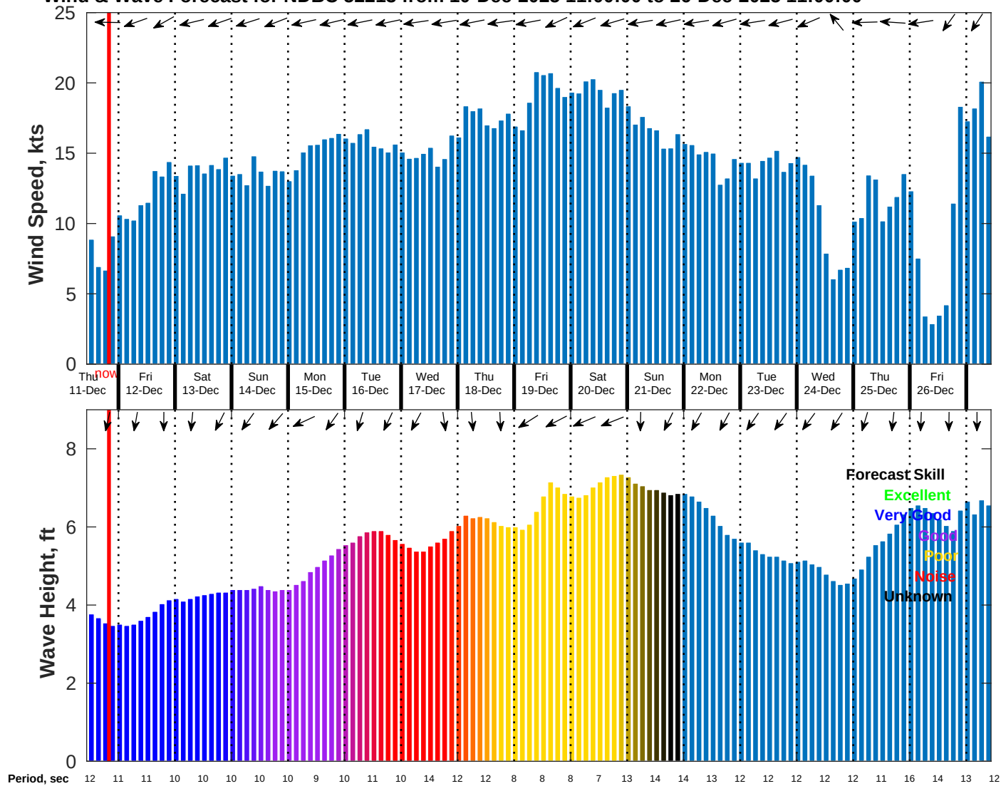
Wind & Wave Forecast for NDBC 52213 from 10-Dec-2025 11:00:00 to 26-Dec-2025 11:00:00
