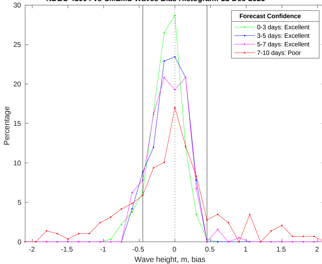
NDBC 41004 vs CMEMS Waves Bias Histogram: 11-Dec-2025
