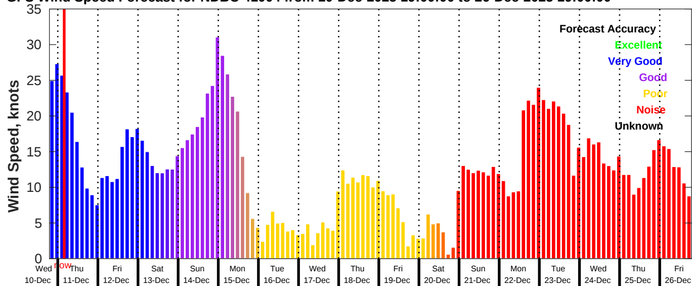
GFS Wind Speed Forecast for NDBC 41004 from 10-Dec-2025 19:00:00 to 26-Dec-2025 19:00:00
