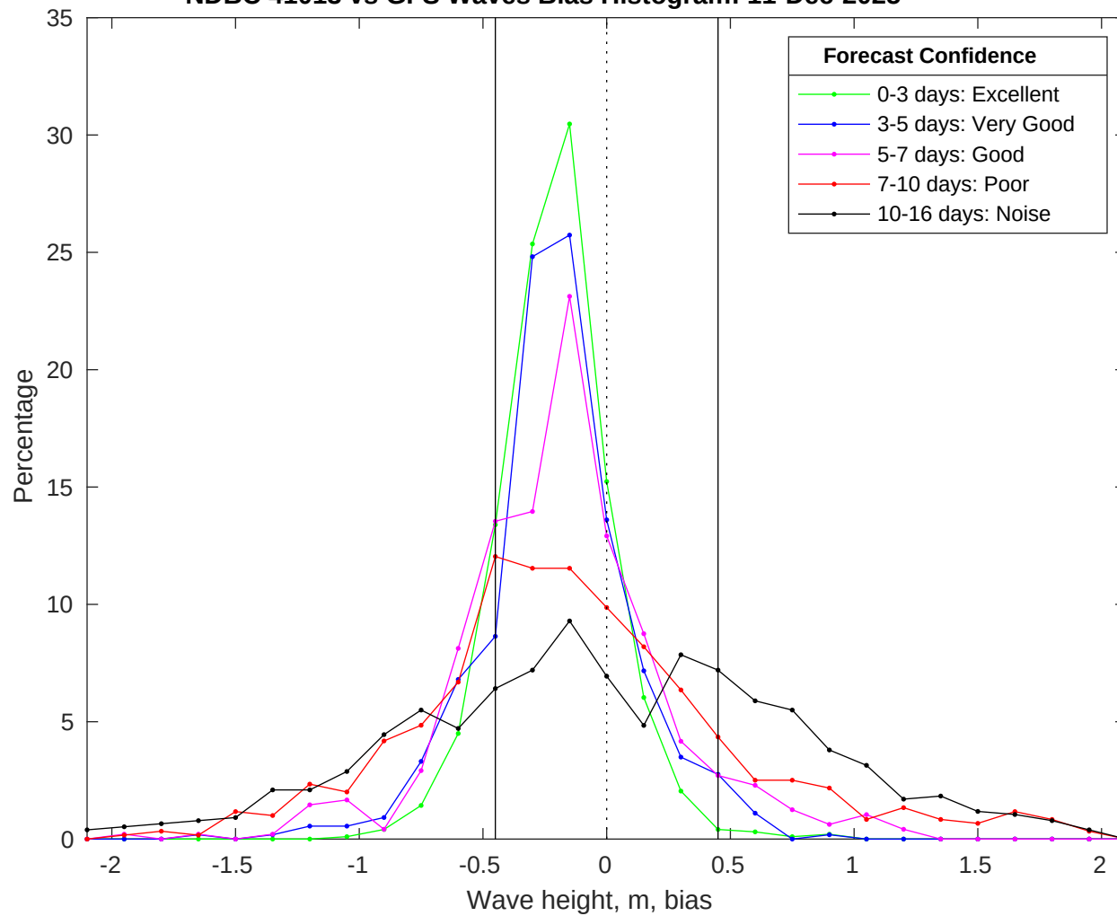
NDBC 41013 vs GFS Waves Bias Histogram: 11-Dec-2025
