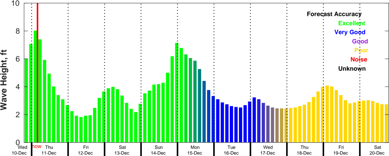
CMEMS Wave Forecast for NDBC 41013 from 10-Dec-2025 19:00:00 to 20-Dec-2025 19:00:00
