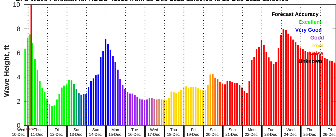
GFS Wave Forecast for NDBC 41013 from 10-Dec-2025 19:00:00 to 26-Dec-2025 19:00:00
