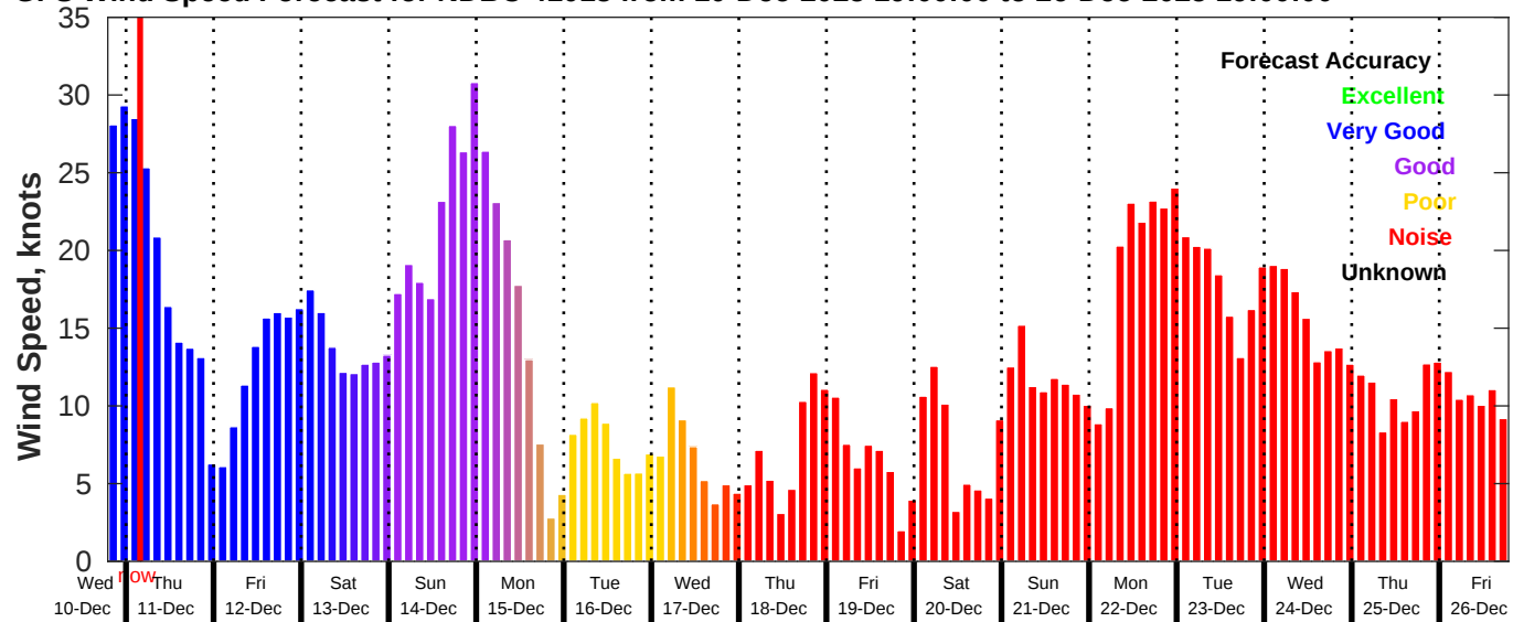
GFS Wind Speed Forecast for NDBC 41013 from 10-Dec-2025 19:00:00 to 26-Dec-2025 19:00:00
