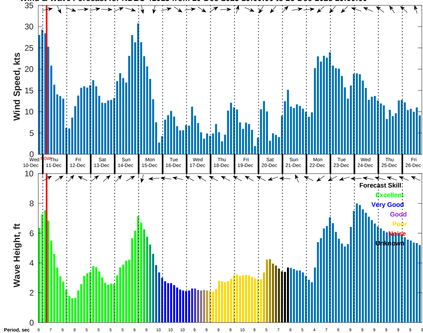
Wind & Wave Forecast for NDBC 41013 from 10-Dec-2025 19:00:00 to 26-Dec-2025 19:00:00
