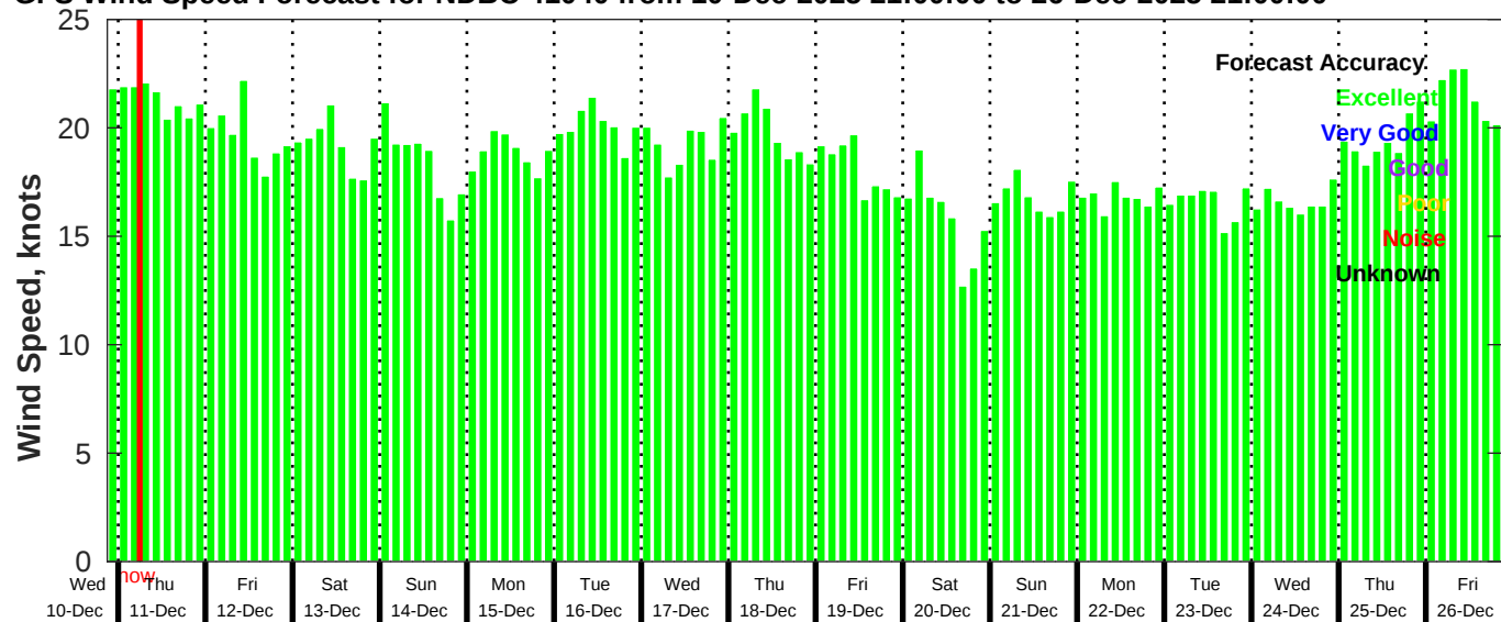
GFS Wind Speed Forecast for NDBC 41040 from 10-Dec-2025 21:00:00 to 26-Dec-2025 21:00:00
