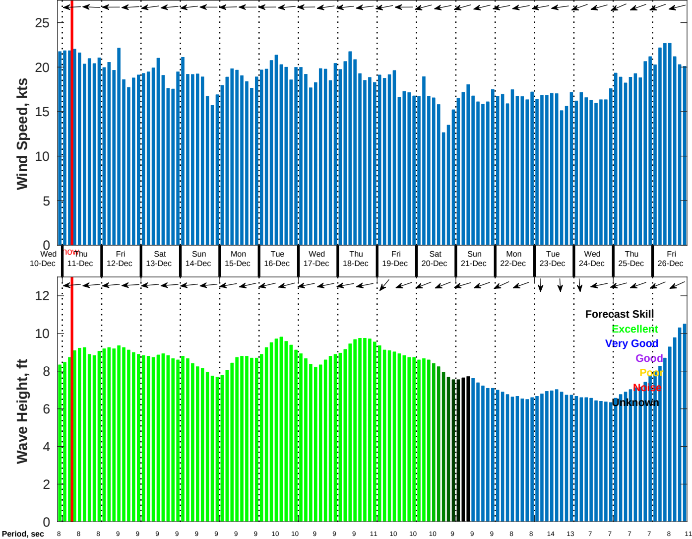
Wind & Wave Forecast for NDBC 41040 from 10-Dec-2025 21:00:00 to 26-Dec-2025 21:00:00
