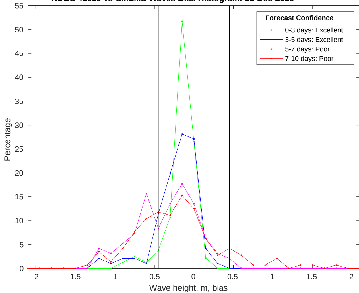
NDBC 42019 vs CMEMS Waves Bias Histogram: 11-Dec-2025
