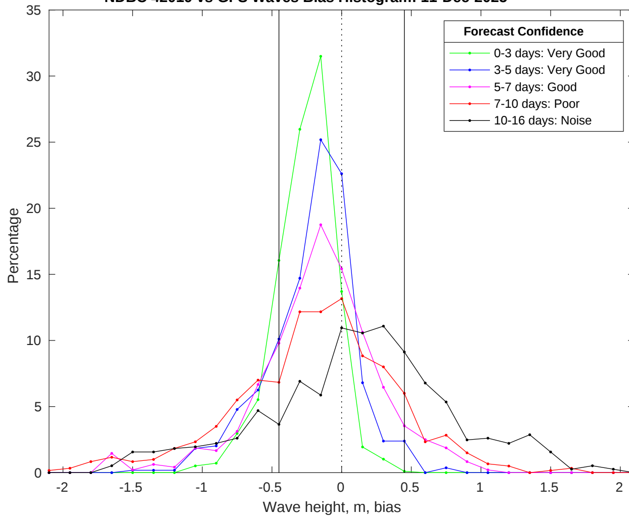
NDBC 42019 vs GFS Waves Bias Histogram: 11-Dec-2025
