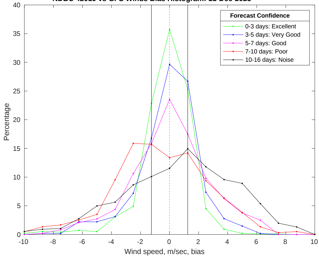
NDBC 42019 vs GFS Winds Bias Histogram: 11-Dec-2025
