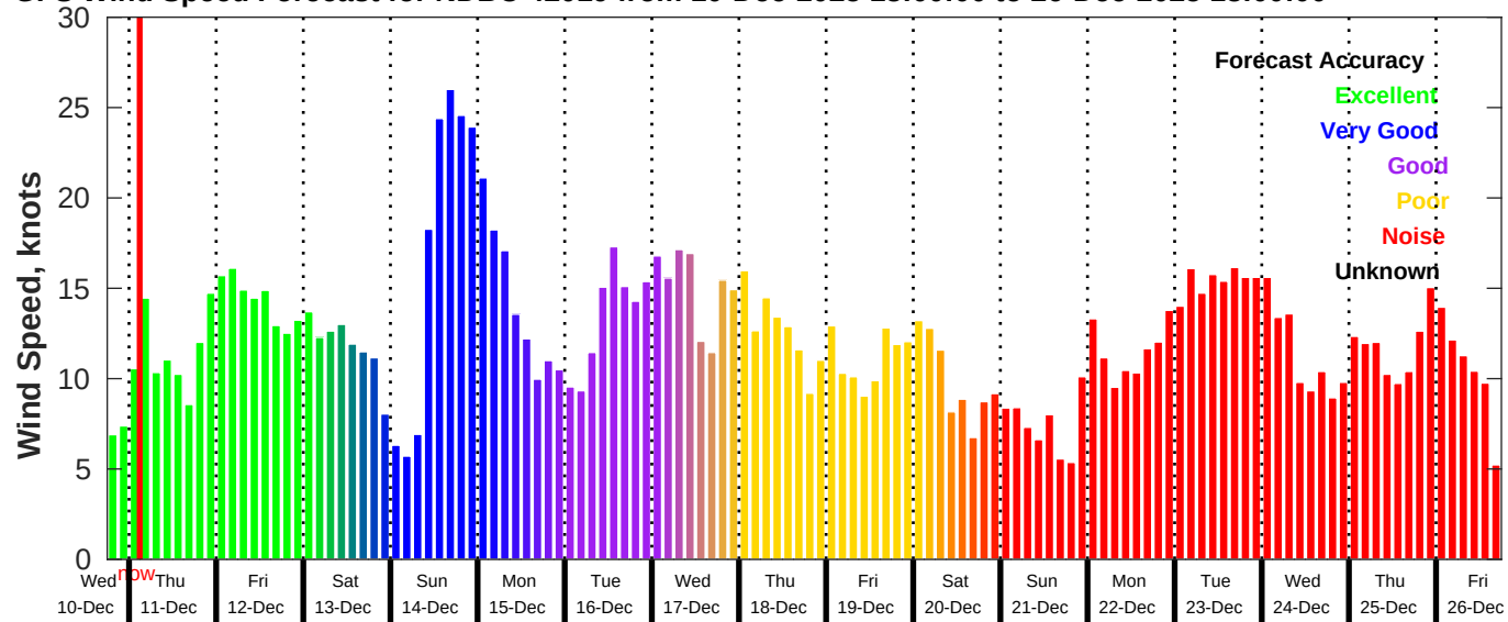
GFS Wind Speed Forecast for NDBC 42019 from 10-Dec-2025 18:00:00 to 26-Dec-2025 18:00:00
