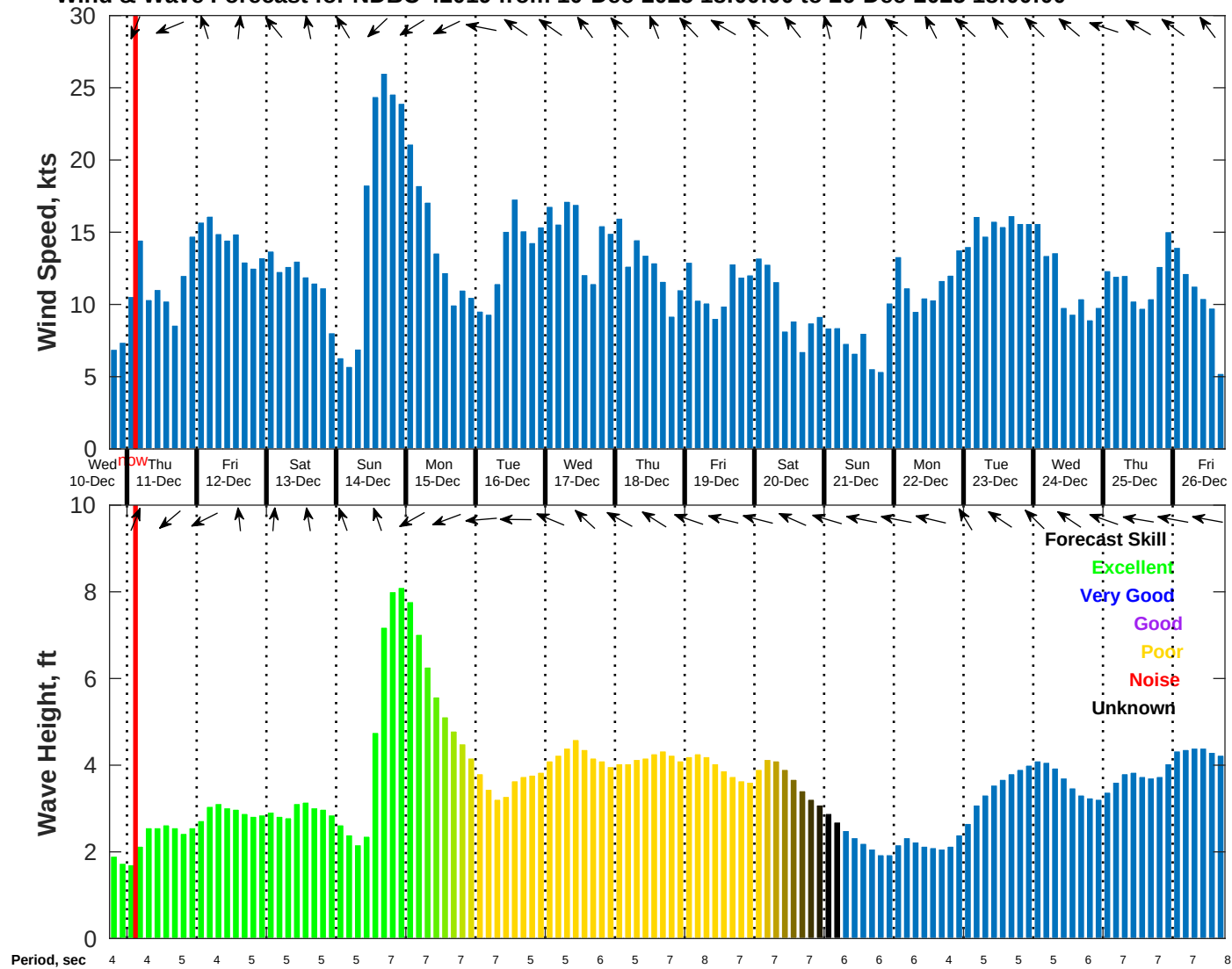
Wind & Wave Forecast for NDBC 42019 from 10-Dec-2025 18:00:00 to 26-Dec-2025 18:00:00
