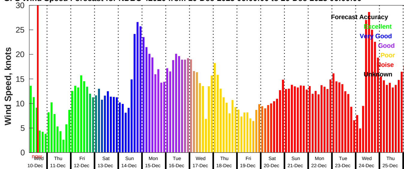
GFS Wind Speed Forecast for NDBC 42020 from 10-Dec-2025 06:00:00 to 26-Dec-2025 06:00:00
