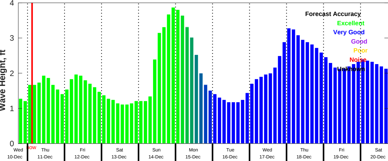
CMEMS Wave Forecast for NDBC 42035 from 10-Dec-2025 18:00:00 to 20-Dec-2025 18:00:00
