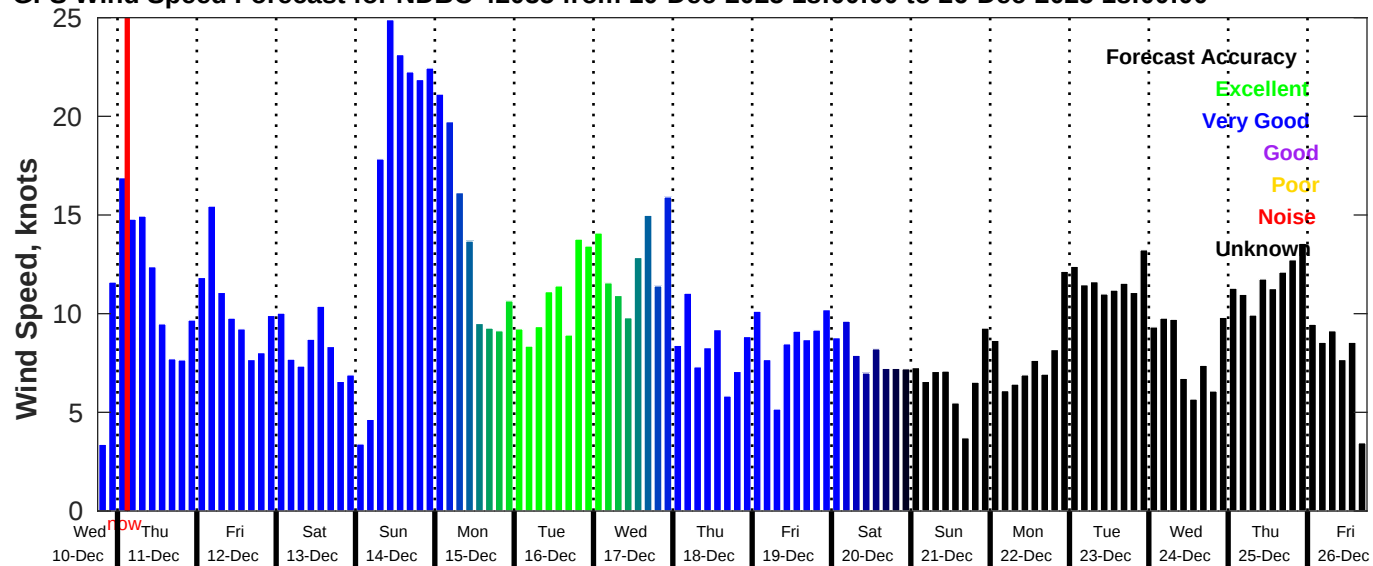
GFS Wind Speed Forecast for NDBC 42035 from 10-Dec-2025 18:00:00 to 26-Dec-2025 18:00:00
