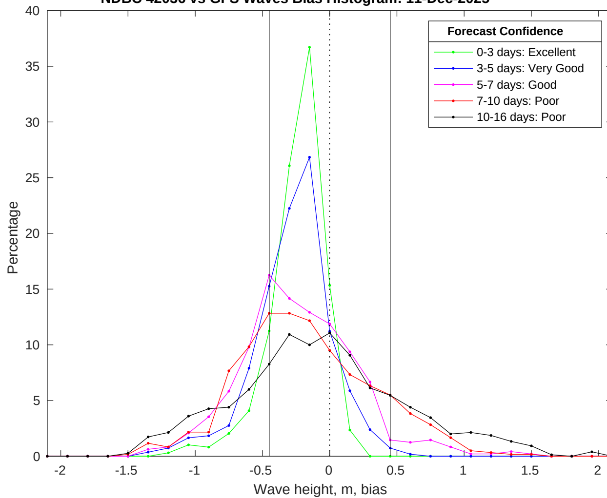
NDBC 42036 vs GFS Waves Bias Histogram: 11-Dec-2025
