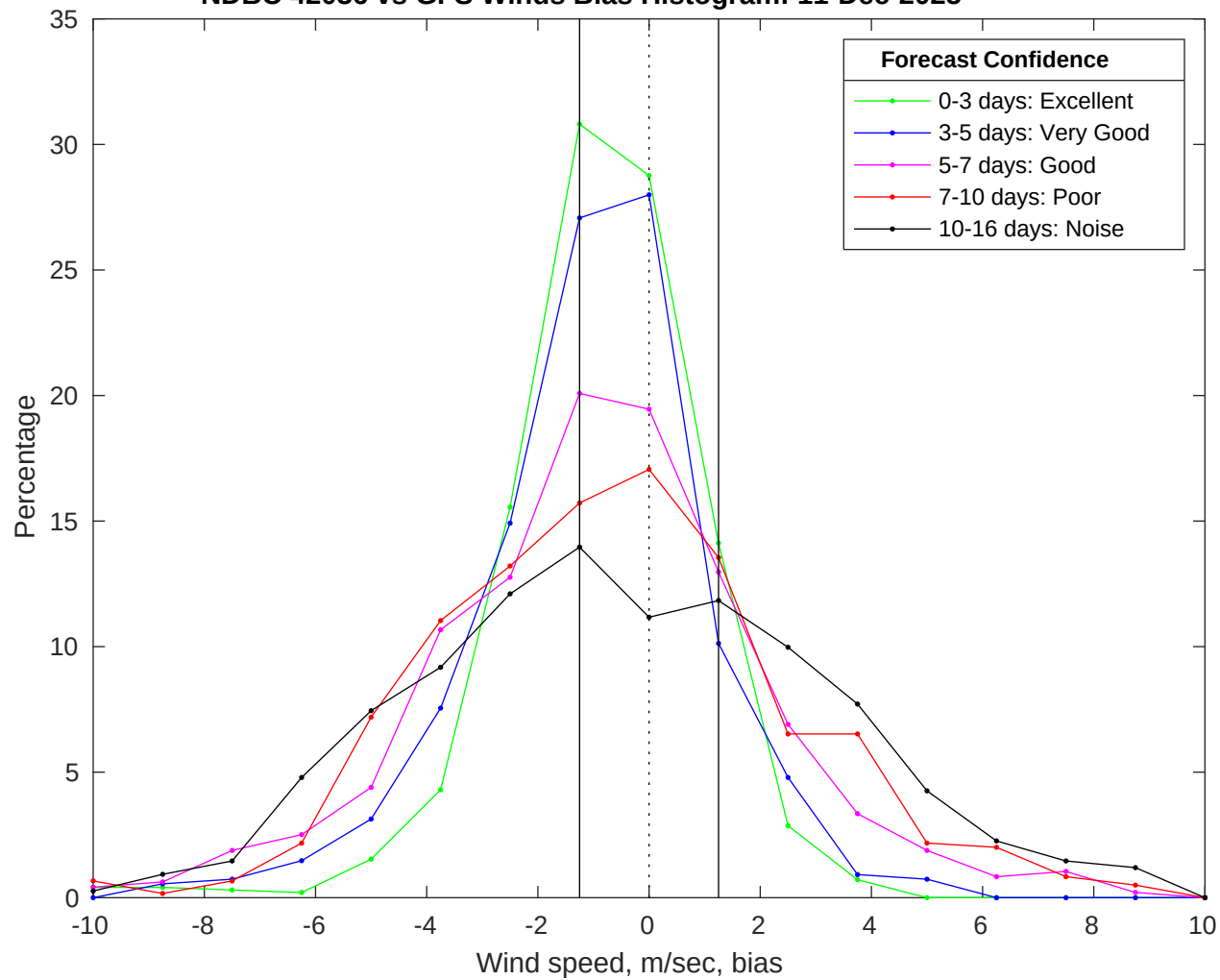
NDBC 42036 vs GFS Winds Bias Histogram: 11-Dec-2025
