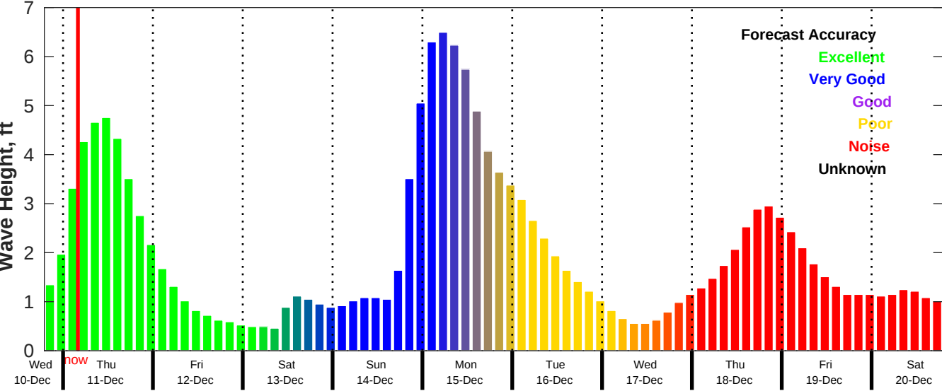
CMEMS Wave Forecast for NDBC 42036 from 10-Dec-2025 19:00:00 to 20-Dec-2025 19:00:00
