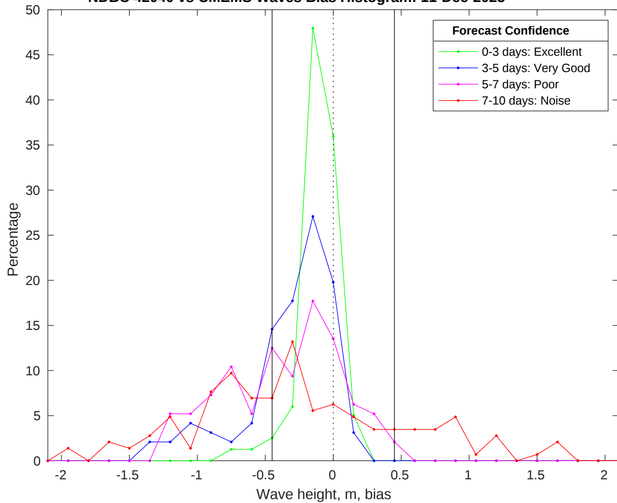
NDBC 42040 vs CMEMS Waves Bias Histogram: 11-Dec-2025
