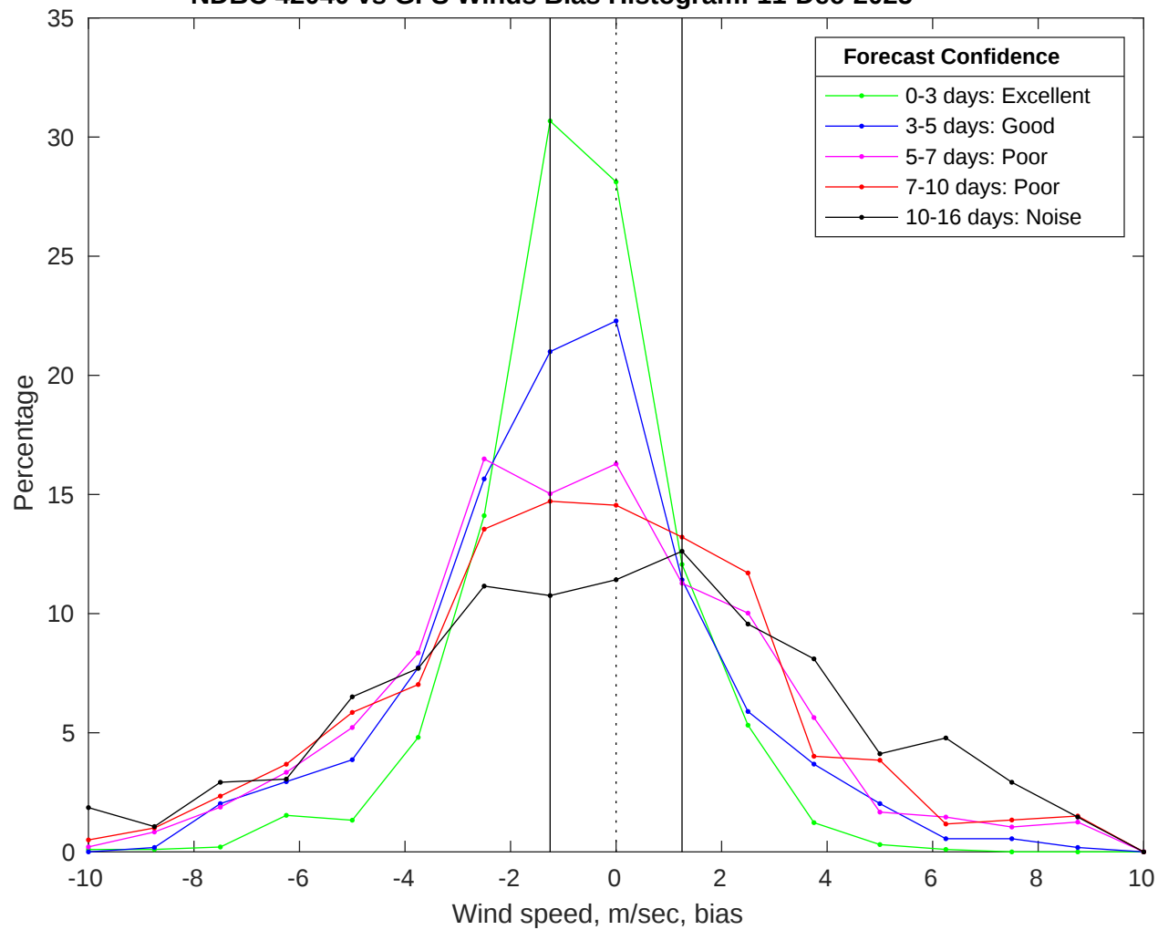
NDBC 42040 vs GFS Winds Bias Histogram: 11-Dec-2025
