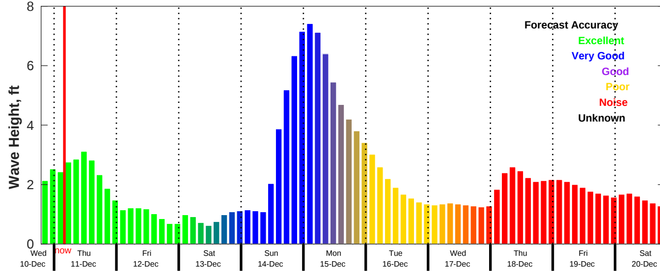
CMEMS Wave Forecast for NDBC 42040 from 10-Dec-2025 19:00:00 to 20-Dec-2025 19:00:00
