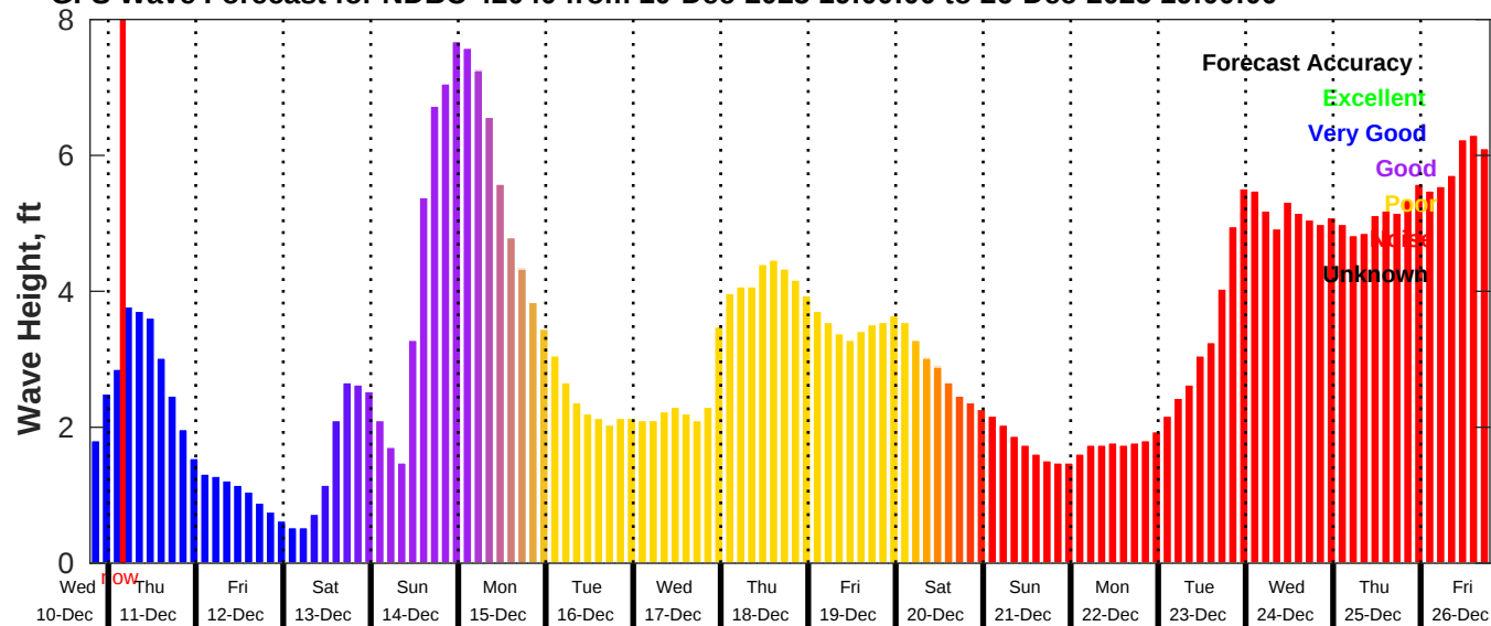
GFS Wave Forecast for NDBC 42040 from 10-Dec-2025 19:00:00 to 26-Dec-2025 19:00:00
