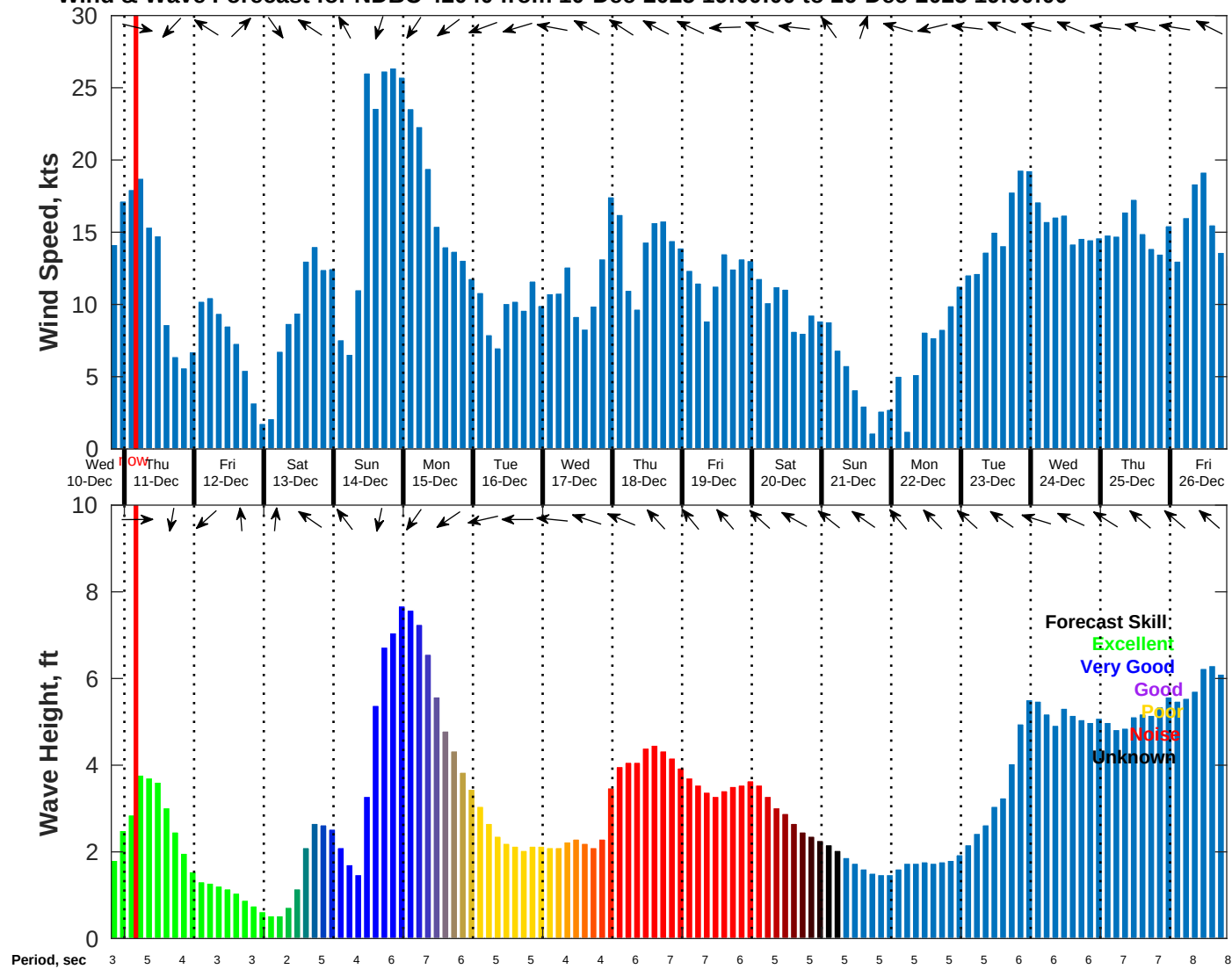
Wind & Wave Forecast for NDBC 42040 from 10-Dec-2025 19:00:00 to 26-Dec-2025 19:00:00
