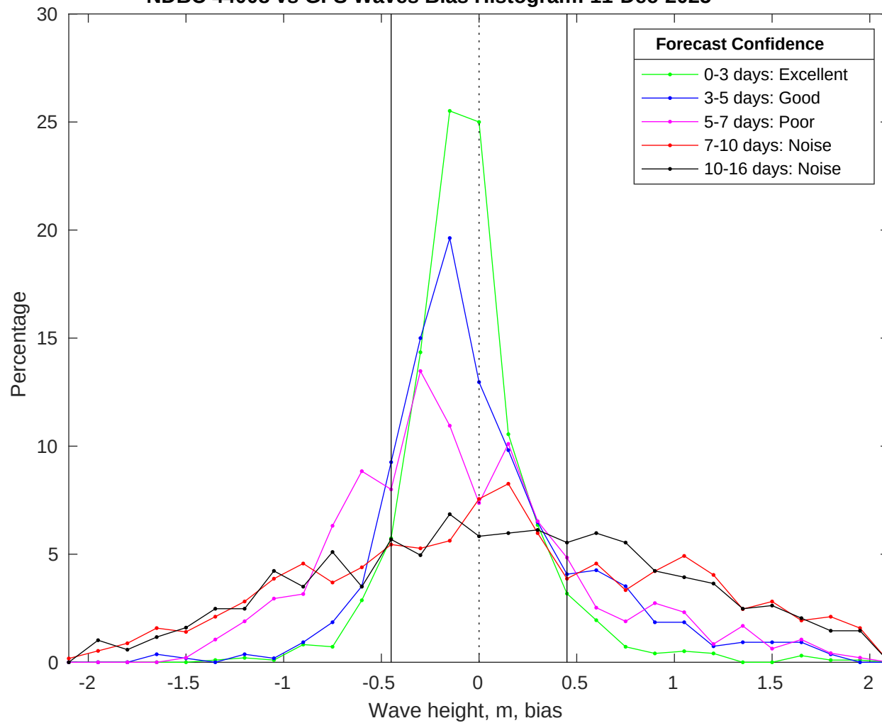
NDBC 44008 vs GFS Waves Bias Histogram: 11-Dec-2025
