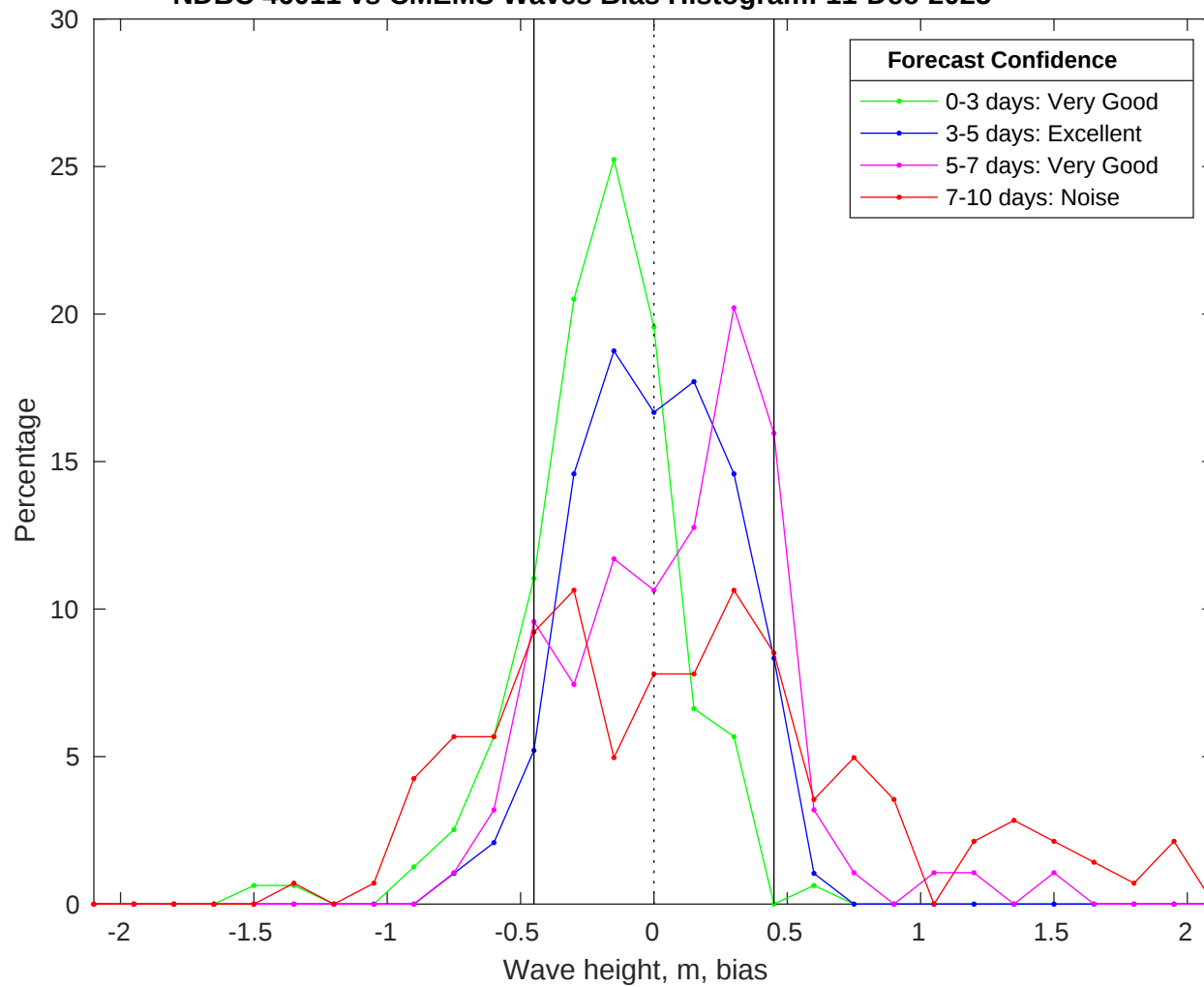
NDBC 46011 vs CMEMS Waves Bias Histogram: 11-Dec-2025
