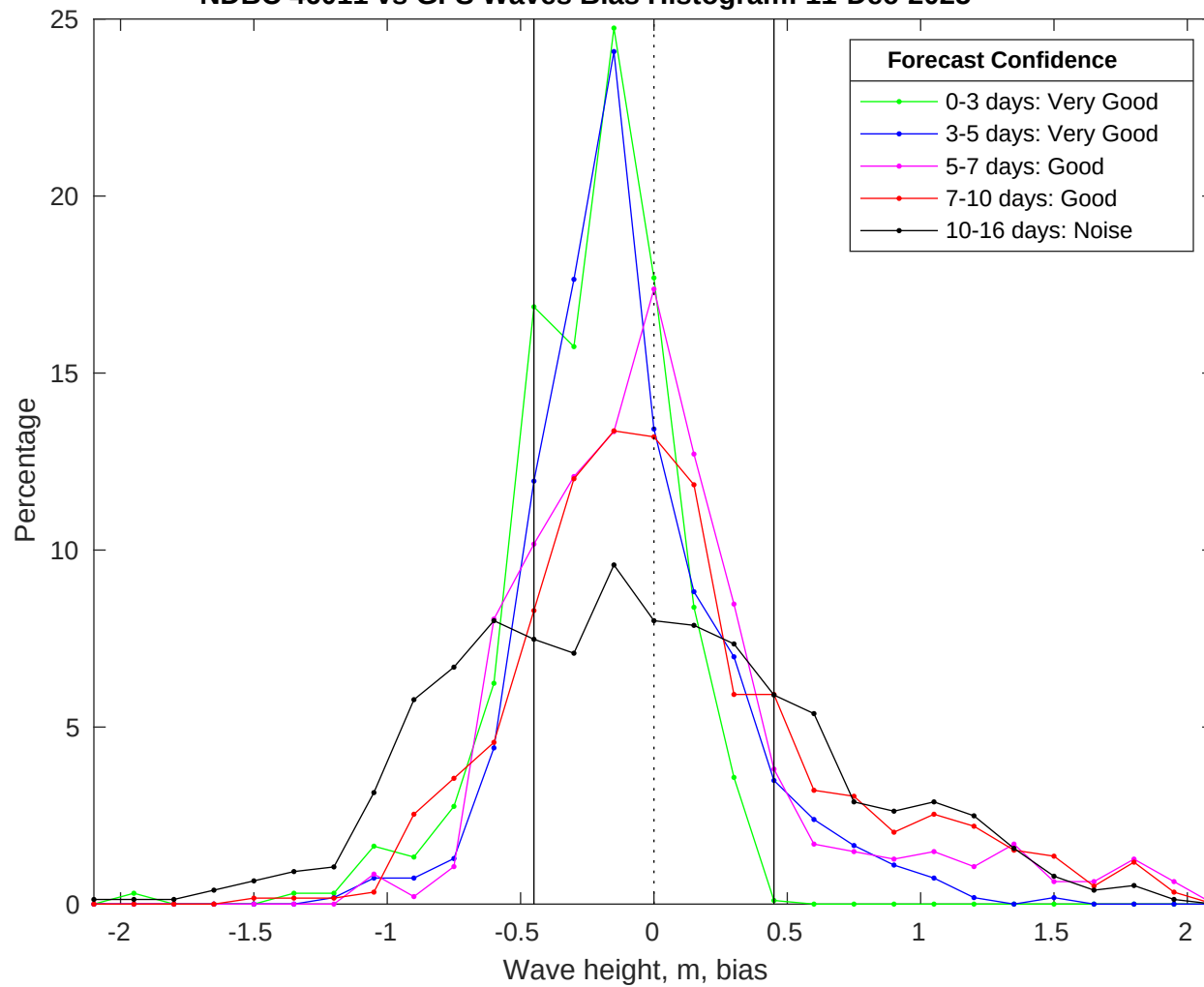
NDBC 46011 vs GFS Waves Bias Histogram: 11-Dec-2025
