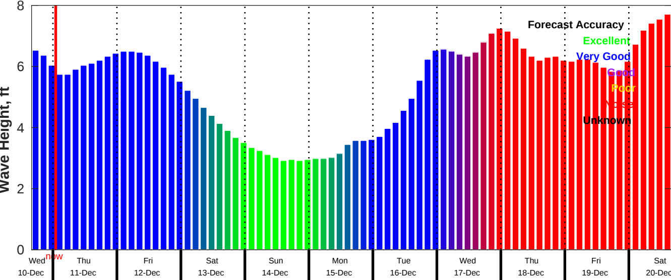
CMEMS Wave Forecast for NDBC 46011 from 10-Dec-2025 16:00:00 to 20-Dec-2025 16:00:00
