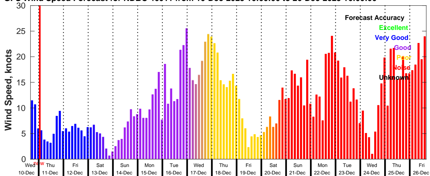
GFS Wind Speed Forecast for NDBC 46011 from 10-Dec-2025 16:00:00 to 26-Dec-2025 16:00:00
