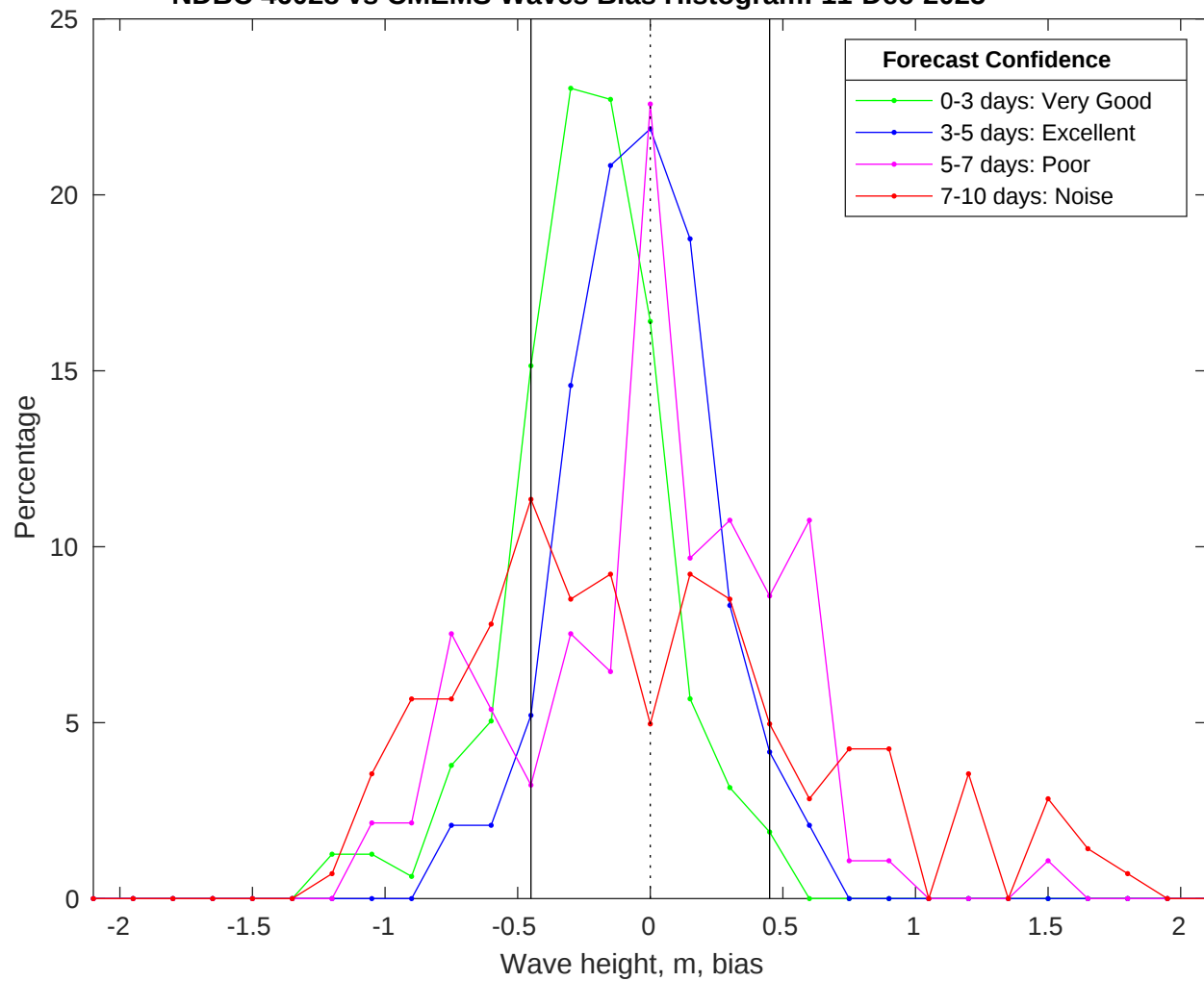
NDBC 46028 vs CMEMS Waves Bias Histogram: 11-Dec-2025
