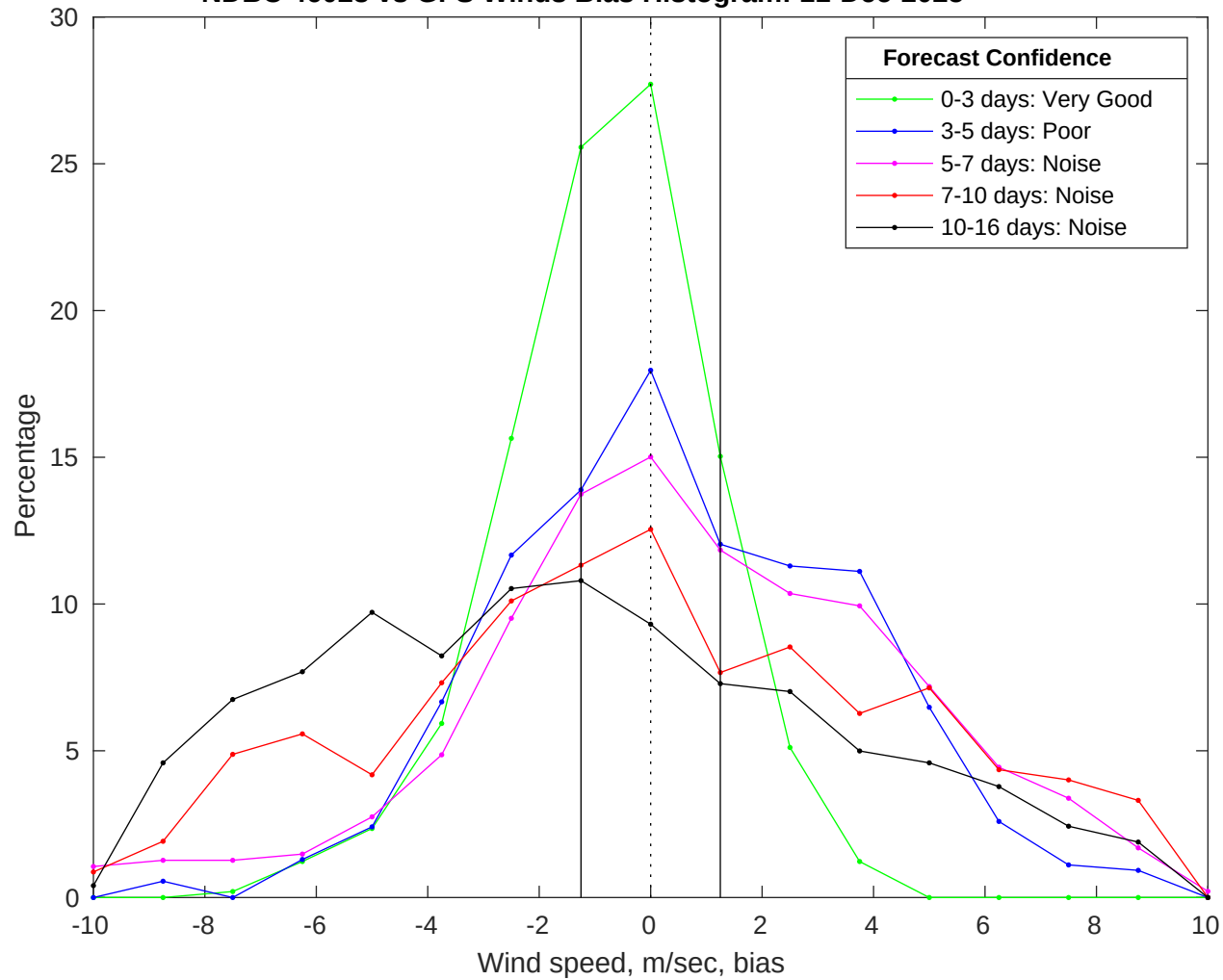
NDBC 46028 vs GFS Winds Bias Histogram: 11-Dec-2025
