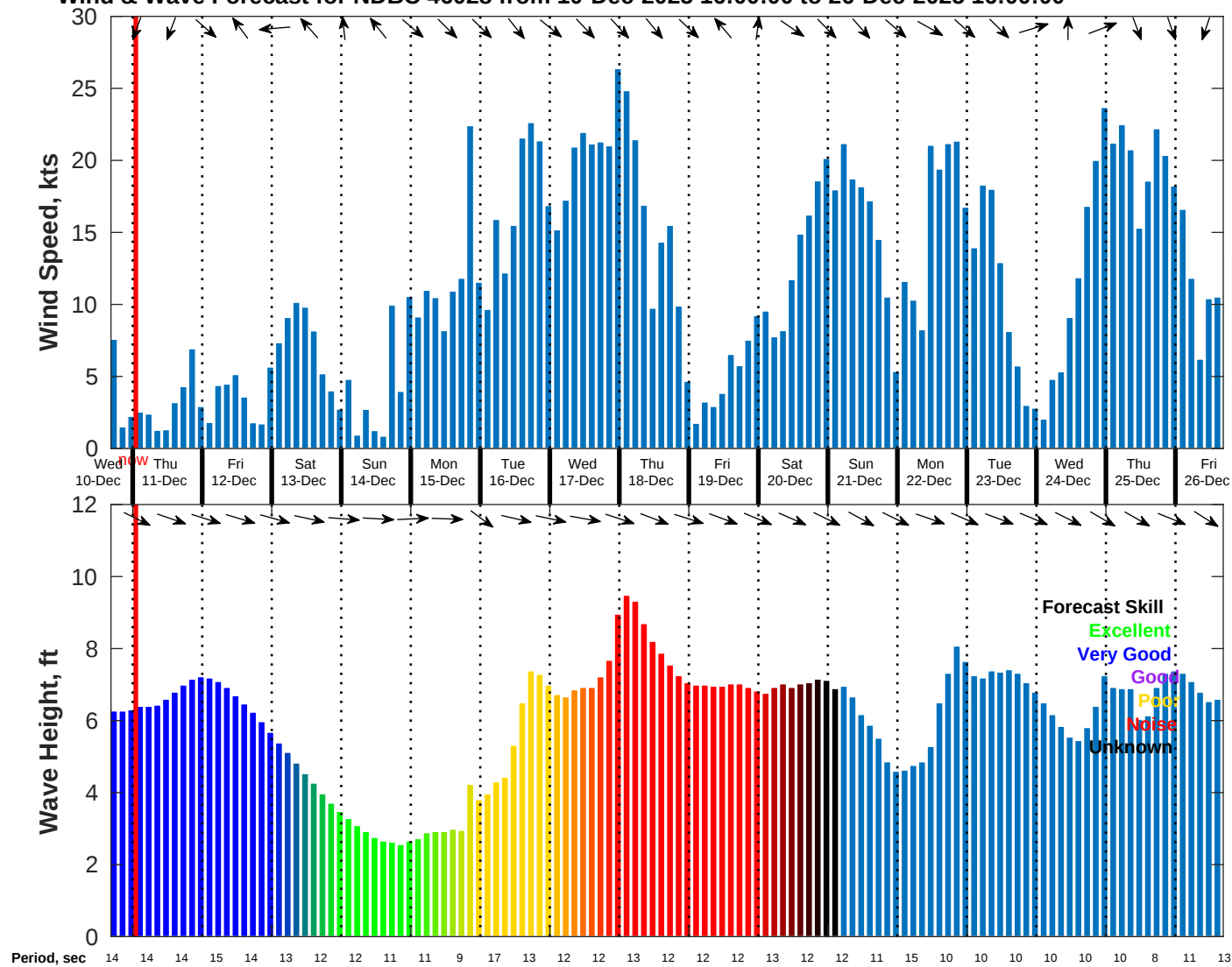
Wind & Wave Forecast for NDBC 46028 from 10-Dec-2025 16:00:00 to 26-Dec-2025 16:00:00
