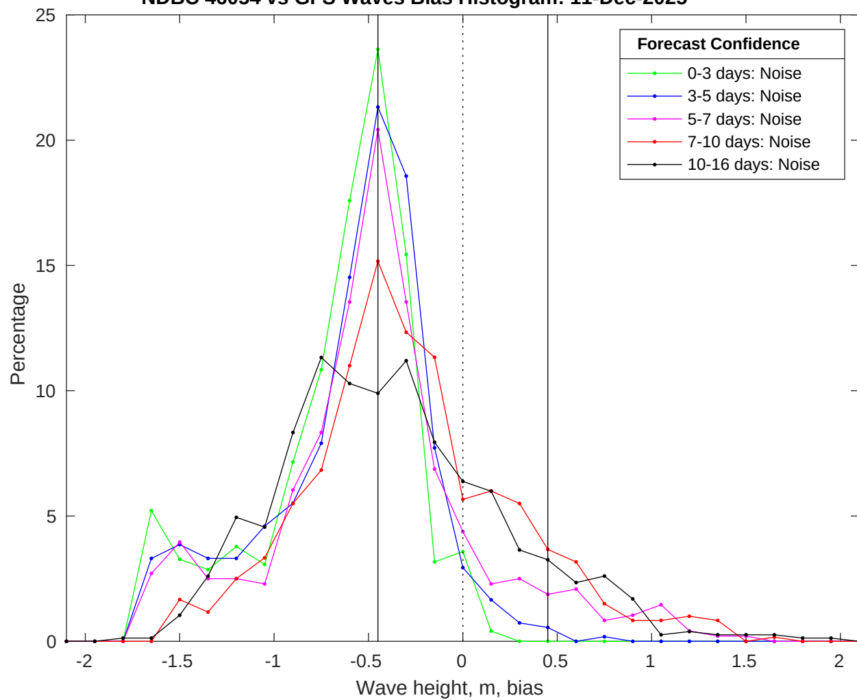
NDBC 46054 vs GFS Waves Bias Histogram: 11-Dec-2025
