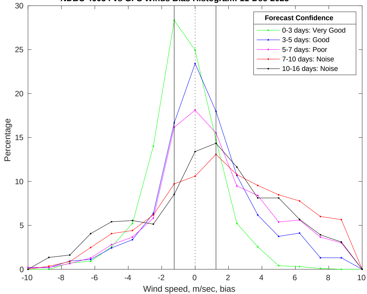
NDBC 46054 vs GFS Winds Bias Histogram: 11-Dec-2025
