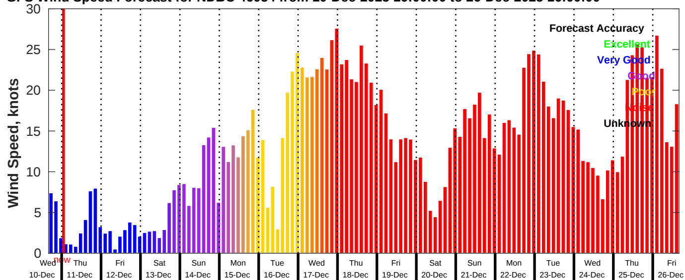
GFS Wind Speed Forecast for NDBC 46054 from 10-Dec-2025 16:00:00 to 26-Dec-2025 16:00:00
