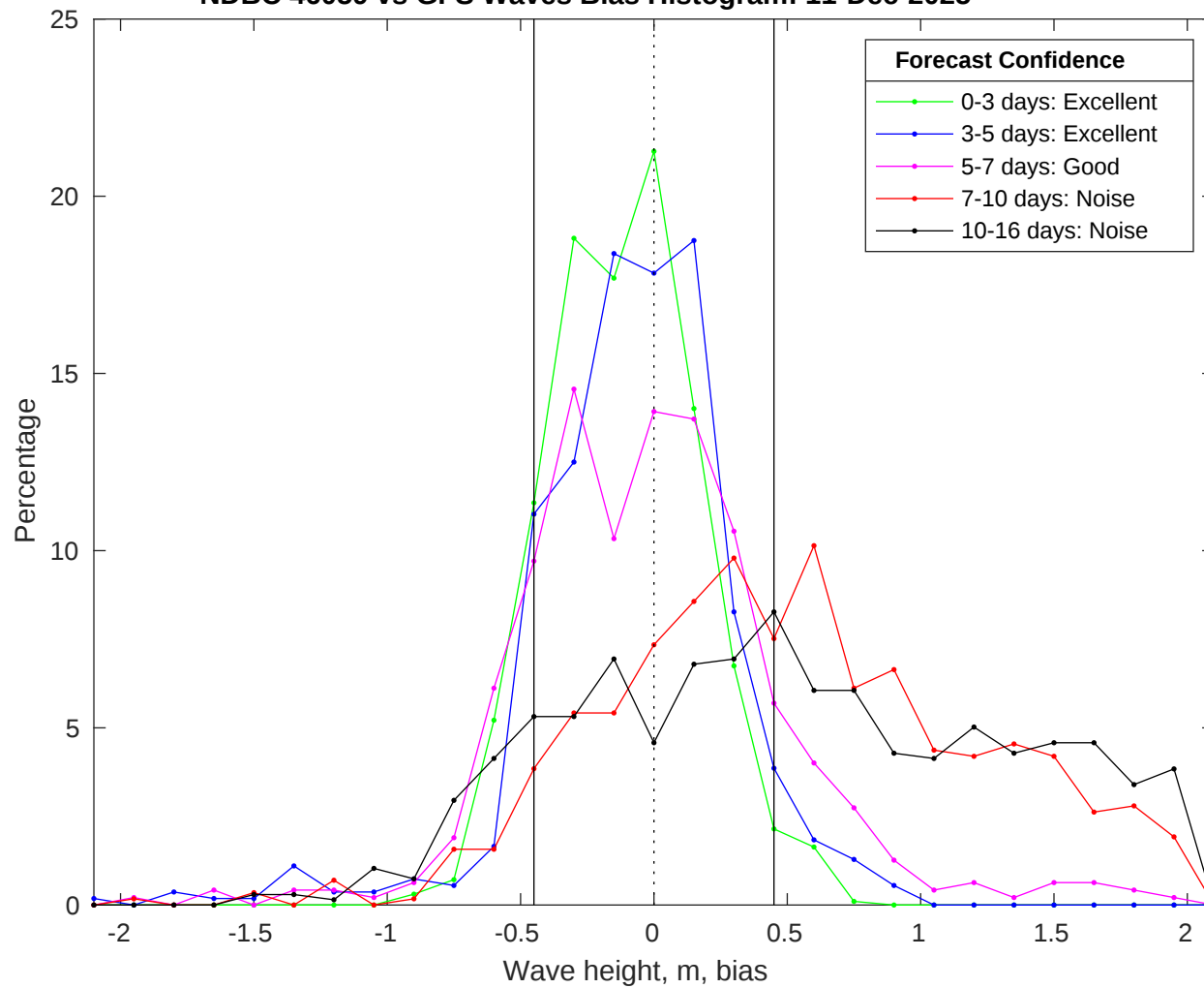
NDBC 46059 vs GFS Waves Bias Histogram: 11-Dec-2025
