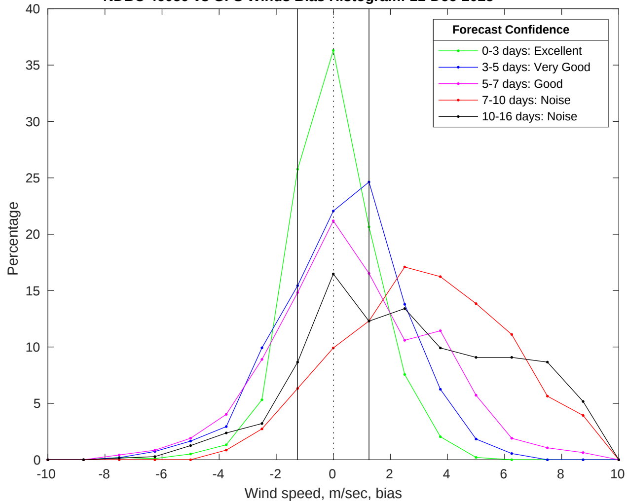
NDBC 46059 vs GFS Winds Bias Histogram: 11-Dec-2025
