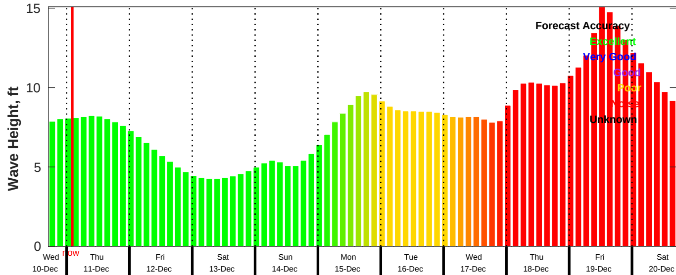
CMEMS Wave Forecast for NDBC 46059 from 10-Dec-2025 17:00:00 to 20-Dec-2025 17:00:00
