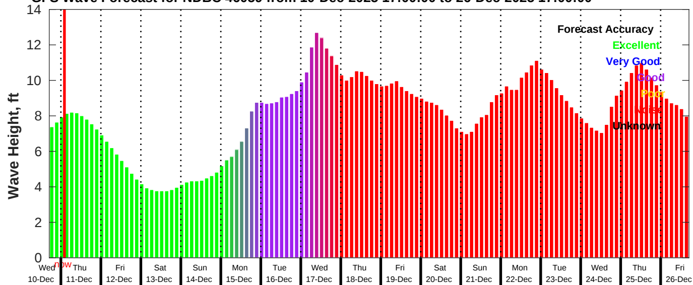
GFS Wave Forecast for NDBC 46059 from 10-Dec-2025 17:00:00 to 26-Dec-2025 17:00:00
