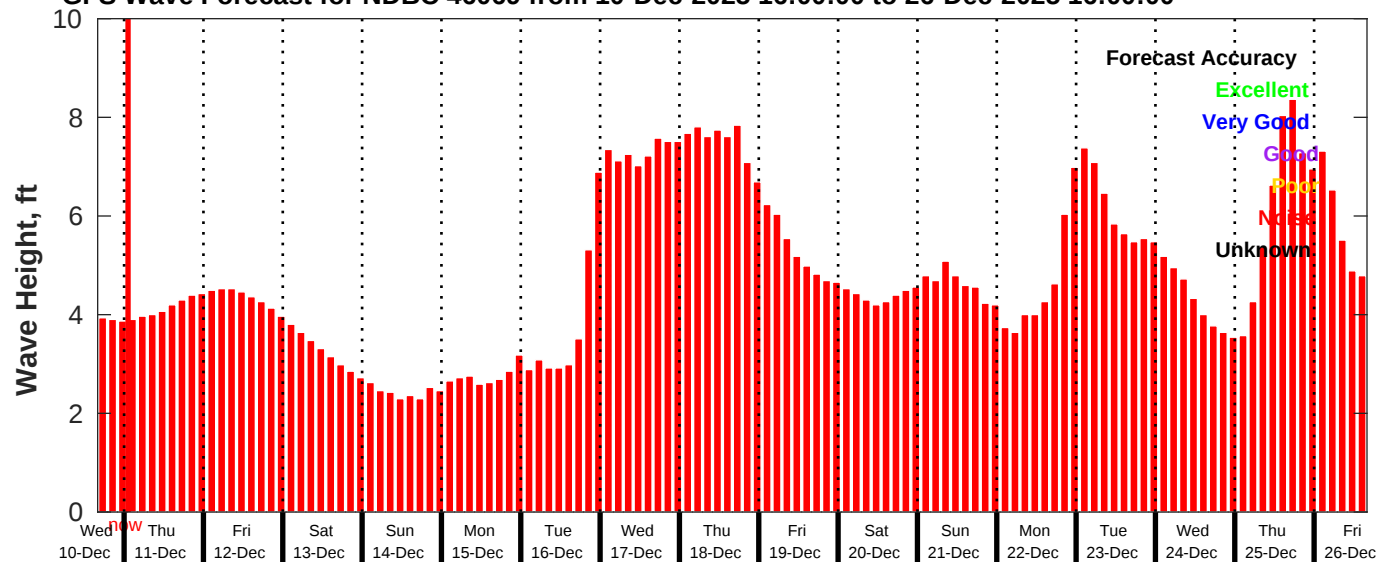
GFS Wave Forecast for NDBC 46069 from 10-Dec-2025 16:00:00 to 26-Dec-2025 16:00:00
