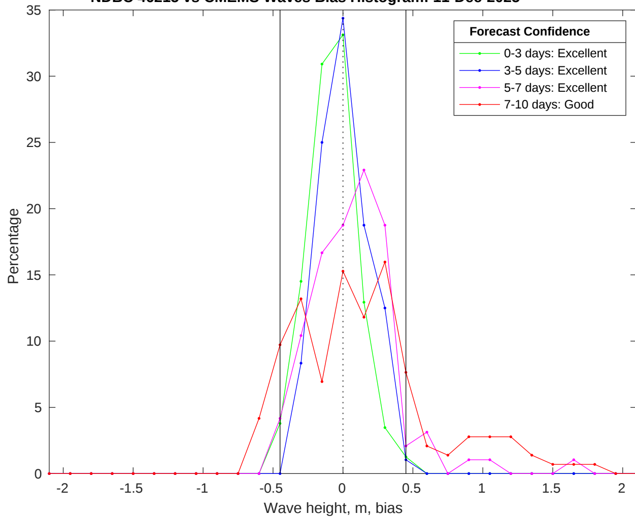
NDBC 46215 vs CMEMS Waves Bias Histogram: 11-Dec-2025
