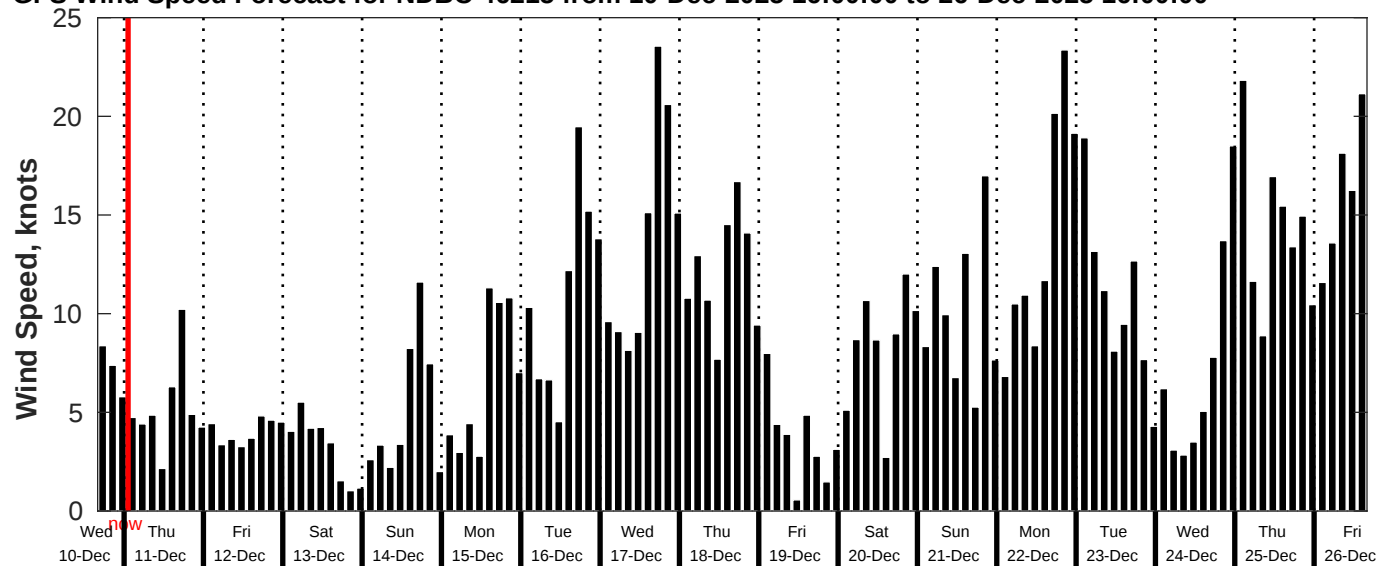
GFS Wind Speed Forecast for NDBC 46215 from 10-Dec-2025 16:00:00 to 26-Dec-2025 16:00:00
