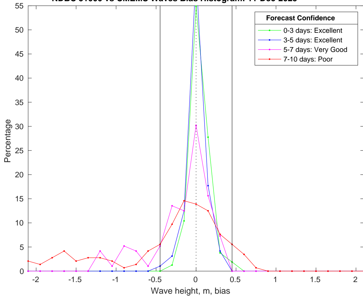
NDBC 51000 vs CMEMS Waves Bias Histogram: 11-Dec-2025
