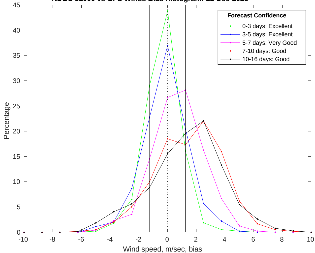
NDBC 51000 vs GFS Winds Bias Histogram: 11-Dec-2025
