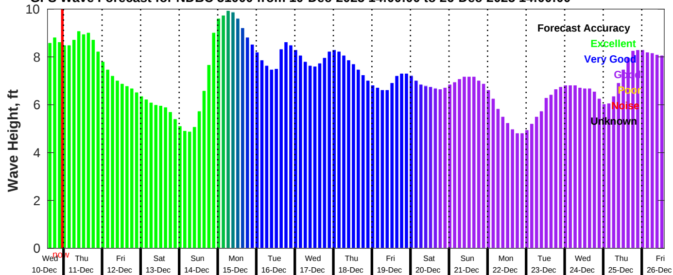
GFS Wave Forecast for NDBC 51000 from 10-Dec-2025 14:00:00 to 26-Dec-2025 14:00:00
