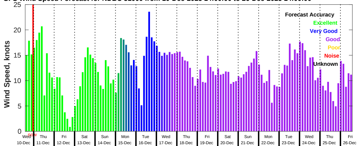
GFS Wind Speed Forecast for NDBC 51000 from 10-Dec-2025 14:00:00 to 26-Dec-2025 14:00:00
