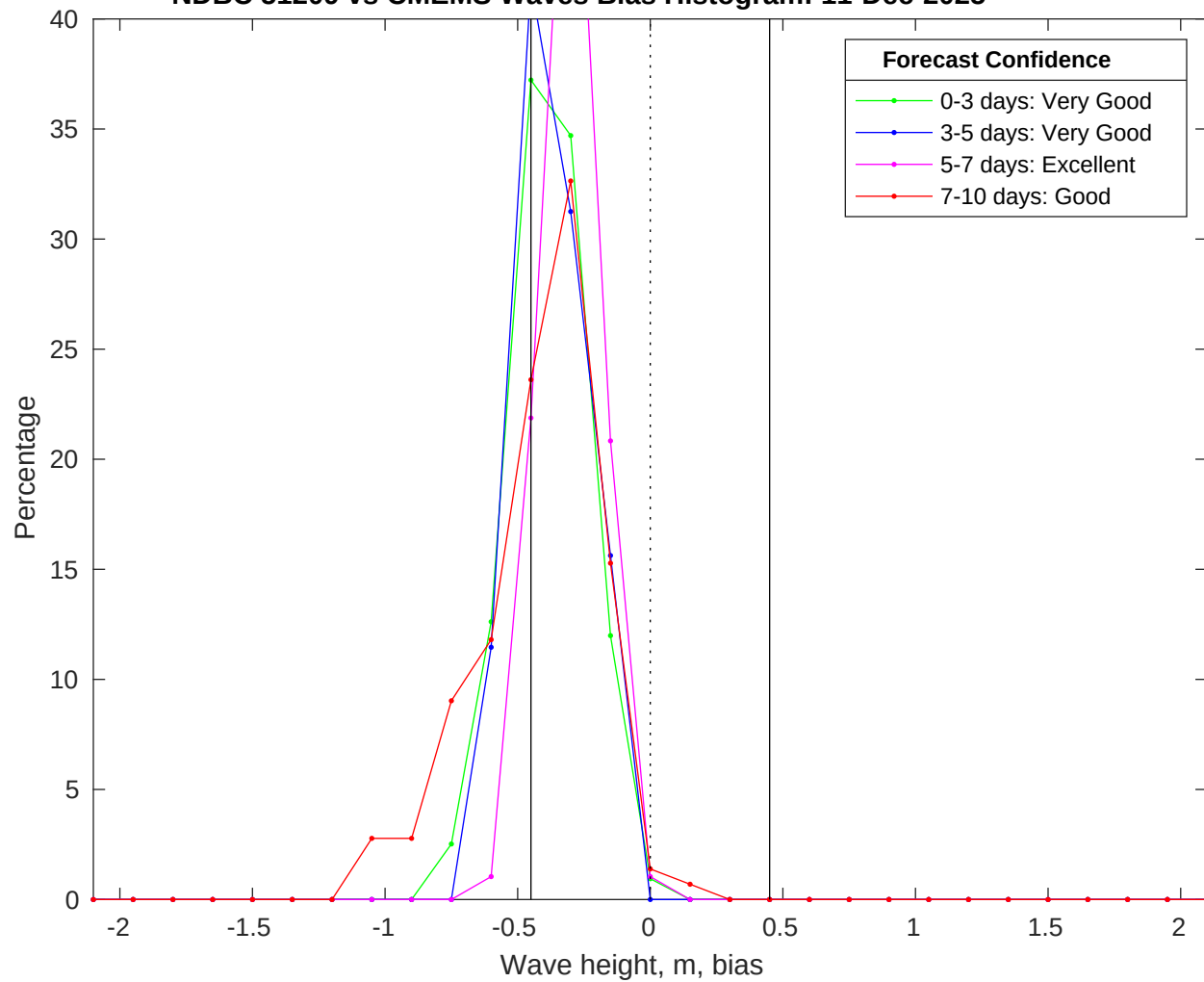
NDBC 51209 vs CMEMS Waves Bias Histogram: 11-Dec-2025
