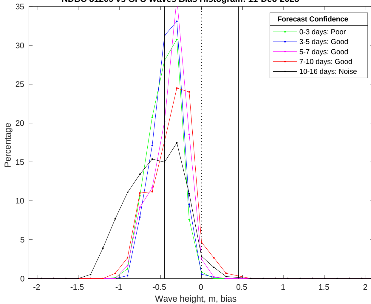
NDBC 51209 vs GFS Waves Bias Histogram: 11-Dec-2025
